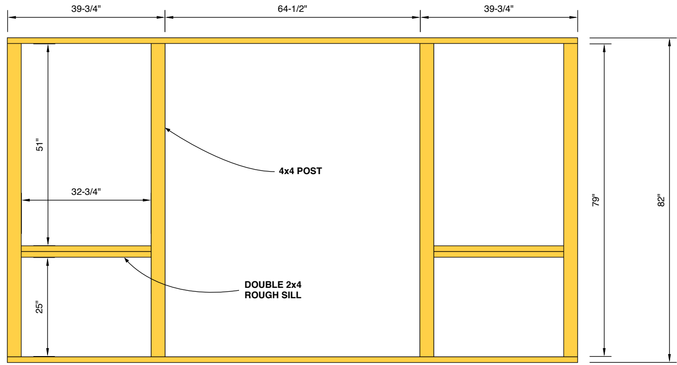
Figure D Front and Back Walls
