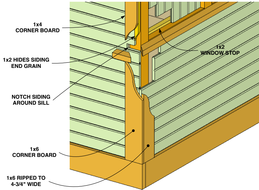
BACK CORNER DETAIL
