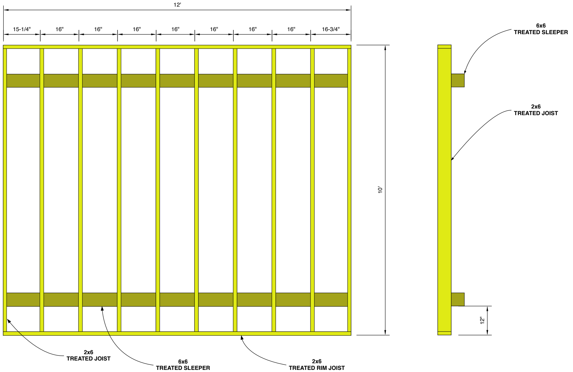
Figure B Floor Framing
