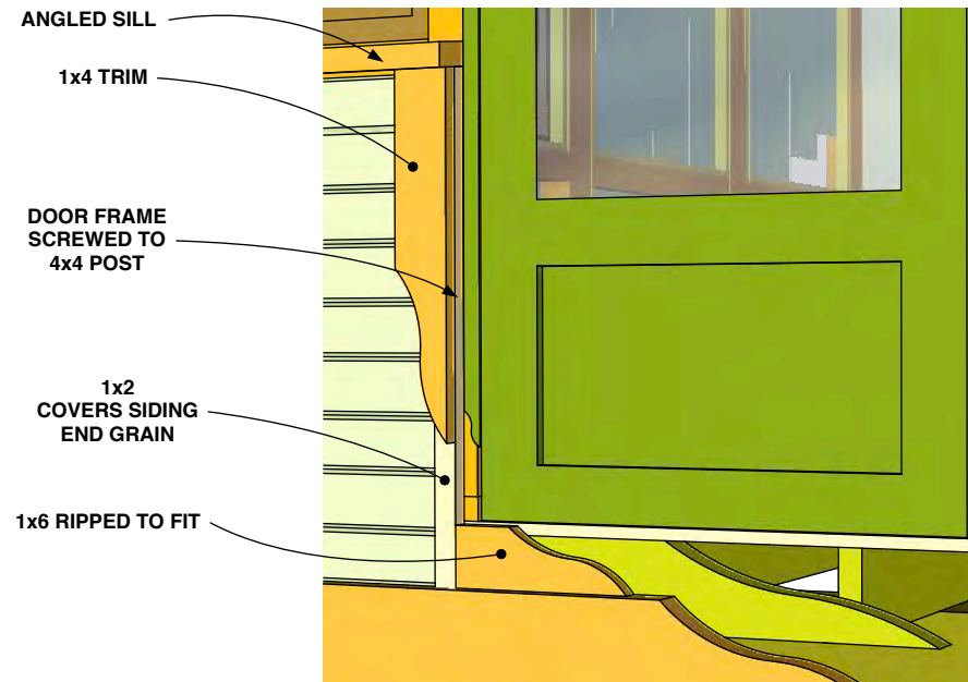
FRONT DOOR DETAIL
