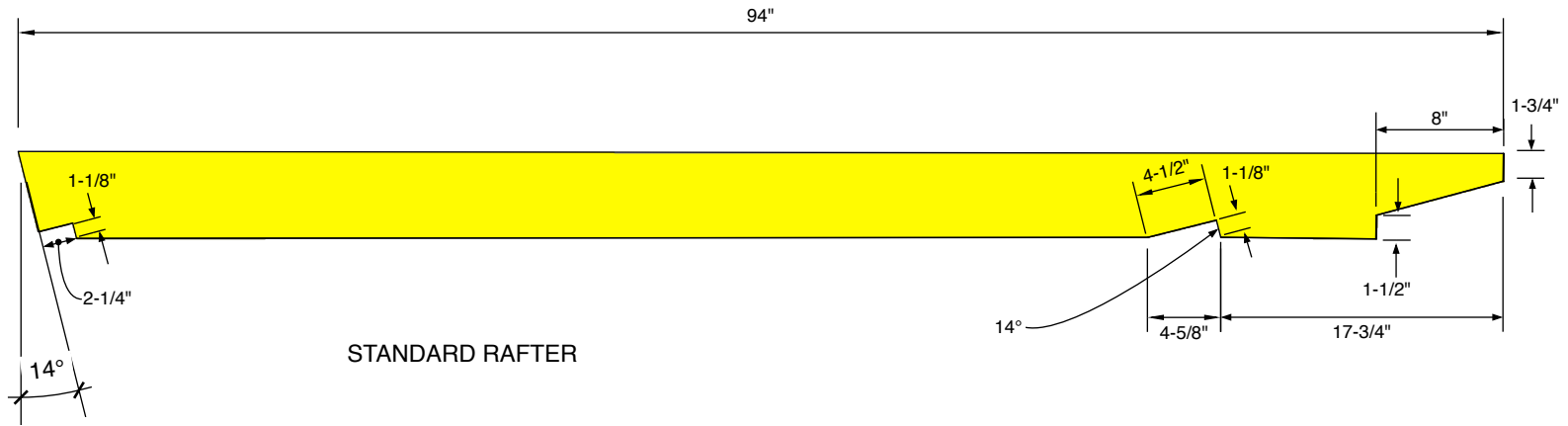
Figure G Rafter Details
